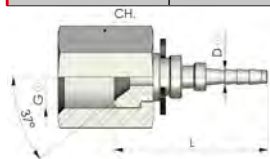
ΘΗΛ. UNF S2
