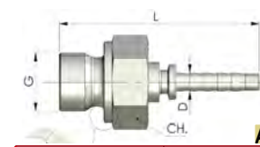
ΘΗΛ. INTΣΑΣ BSP S2
